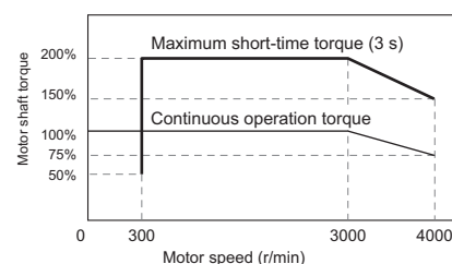
[Operation torque characteristics]
